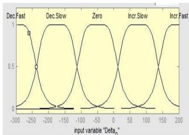
Figure 3.3 Membership function of the DeltaQ input
